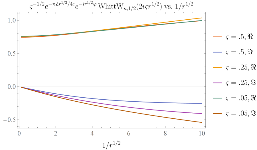
FIGURE 11. The real and imaginary parts of the function \zeta^{-1/2} \exp(-\pi Z r^{1/2}/4\zeta) \exp(-ir^{1/2}\varphi) \text{Whitt}_{\kappa, 1/2}(2i\zeta r^{1/2}) (with the same color scheme as in Figure 10), now plotted as a function of \rho = 1/r^{1/2} , for \zeta \in \{.05, .25, .5\} and Z = 3 .
