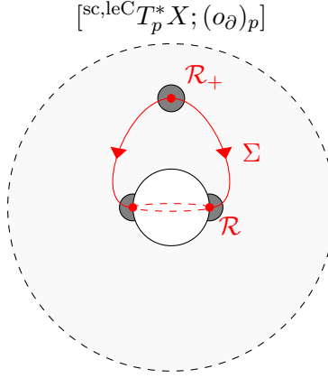
FIGURE 6. The result of blowing up the zero section of {}^{\text{sc,leC}}T_{\partial X}^*X over a fixed point p \in (\partial[0, \bar{x}]_{\text{res}}^{\text{sp}} \setminus \text{zf}^\circ \cup (\text{bf} \cap \text{tf})) \times \partial X , with \Sigma = \text{Char}_{\text{leC}}^{2,0,-2,-1,-3}(\tilde{P}) (which, according to \bar{i} , agrees with \text{Char}_{\text{sc,leC}}^{2,0,-2}(\tilde{P}) away from \text{bf} \cup \text{tf} but is deformed by the blow-up) and the vertical Hamiltonian flow on it indicated. Cf. [Vas21a, Figure 3]. The inner black circle depicts either \text{bf} \cap \text{sf} or \text{tf} \cap \text{ff} , depending on whether \sigma > 0 or \sigma = 0 . Over each p , it is a copy of \mathbb{S}^{n-1} . Its equator is the portion of \mathcal{R} over p . The radial point estimate in §5.3 is used to control the dark gray neighborhood, while elliptic estimates suffice for the rest of \text{bf} \cap \text{sf} or \text{tf} \cap \text{ff} (which is away from \mathcal{R} ).
