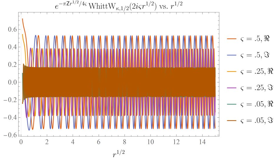
FIGURE 10. The real (in red, orange, and green) and imaginary (in blue, purple, and brown) parts of the function \exp(-\pi Z r^{1/2}/4\zeta) \text{Whitt}_{\kappa, 1/2}(2i\zeta r^{1/2}) as a function of r^{1/2} , for \zeta \in \{.05, .25, .5\} and Z = 3 fixed, where \kappa = -iZr^{1/2}/2\zeta .
