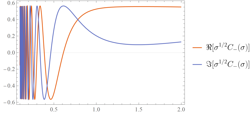
FIGURE 8. The real and imaginary parts of the function C_-(\sigma) defined by eq. (716), rescaled so that the oscillations have constant amplitude.
