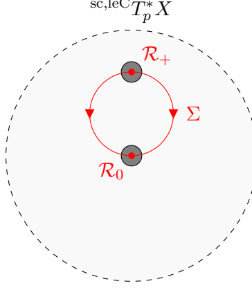
FIGURE 5. Schematic of the proof of eq. (305) when \dim \partial X = 1 . The situation over a point p \in (\partial[0, \bar{x}]_{\text{res}}^{\text{sp}} \setminus \text{zf}^\circ) \times \partial X in the \text{sc,leC} -phase space is illustrated, with \Sigma = \text{Char}_{\text{sc,leC}}^{2,0,-2}(\tilde{P}) in red. There are four subsets of interest: the dark gray neighborhood of \mathcal{R}_+ , controlled using a high regularity radial point estimate, the dark gray neighborhood of \mathcal{R}_0 = o_\partial , controlled using a low regularity radial point estimate (and an elliptic estimate), a neighborhood of the rest of the characteristic set which stays away from \mathcal{R}_+, \mathcal{R}_0 over which we can propagate regularity, and the rest of the cofiber (light gray background), where elliptic estimates apply. Cf. [Mel94, Figure 2]. The direction of the Hamiltonian flow of \tilde{P} is indicated with arrows. (Note that only the “vertical” components of the flow are drawn — the Hamiltonian flow also changes p .)
